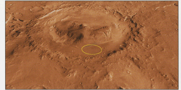
Gale Crater —Curiosity Landing Site
